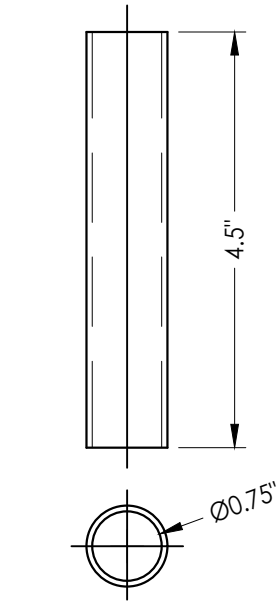
83 SILL TUBE ANCHOR
