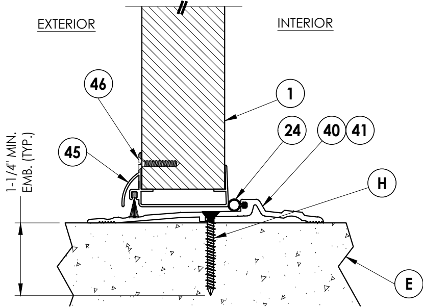
1 VERTICAL CROSS SECTION 5 Outswing configuration
