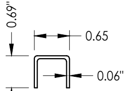
53 GLASS STOP
