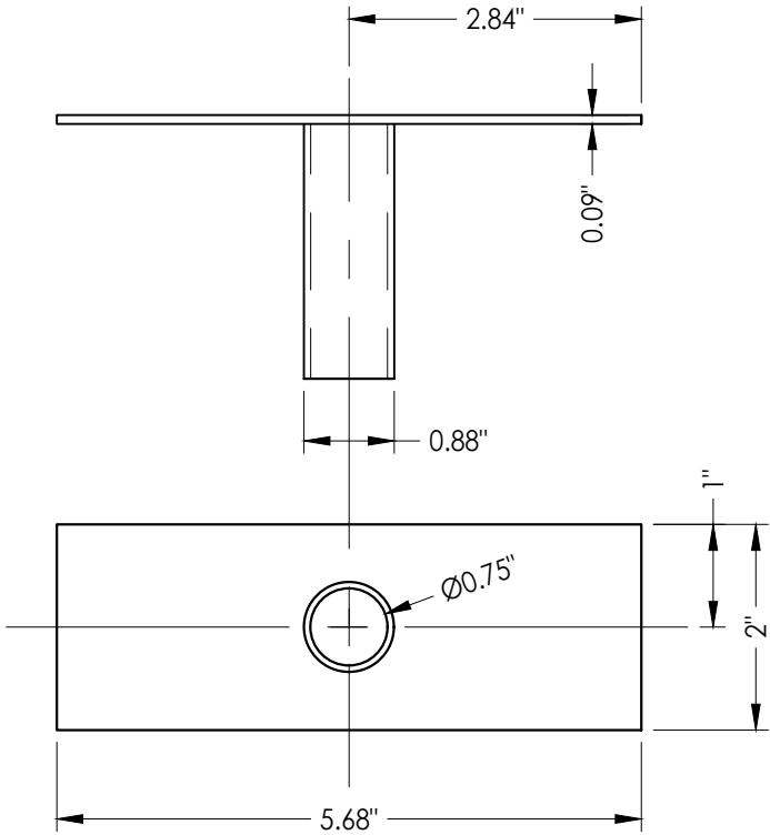
9 TUBE ANCHOR
